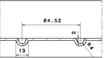
Section view B-B
