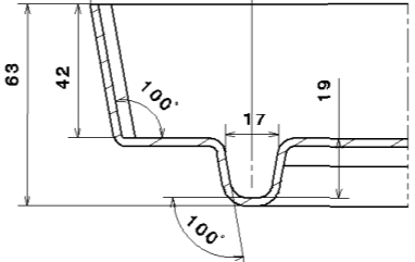
Section view C-C
