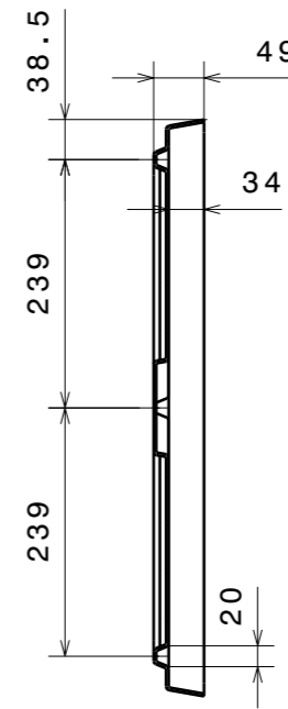
Section view B-B
