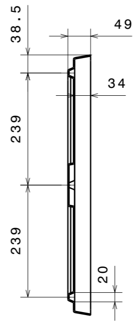
Section view B-B
