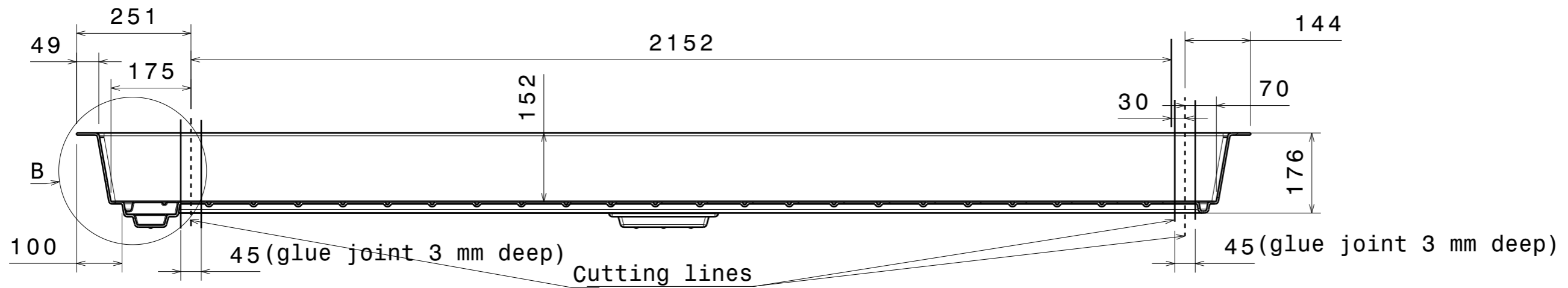
Section view A-A
