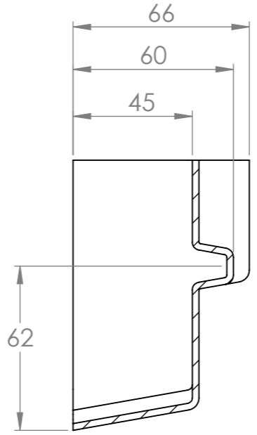
SECTION E-E
